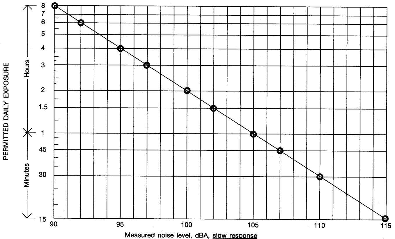
Chart A NOISE EXPOSURE CHART
